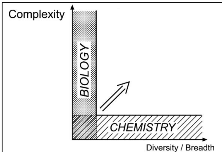
Figure 3: A comparison between Chemistry and Biology with respect to the two parameters: complexity and diversity/breadth
