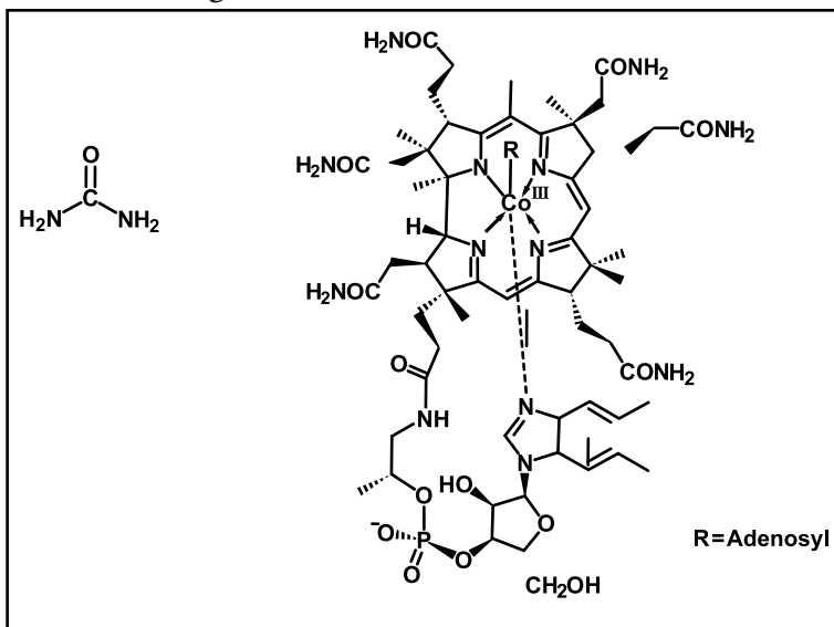
Figure 1: Two milestones in organic synthesis: Urea (left) and Vitamin B 12 (right)
