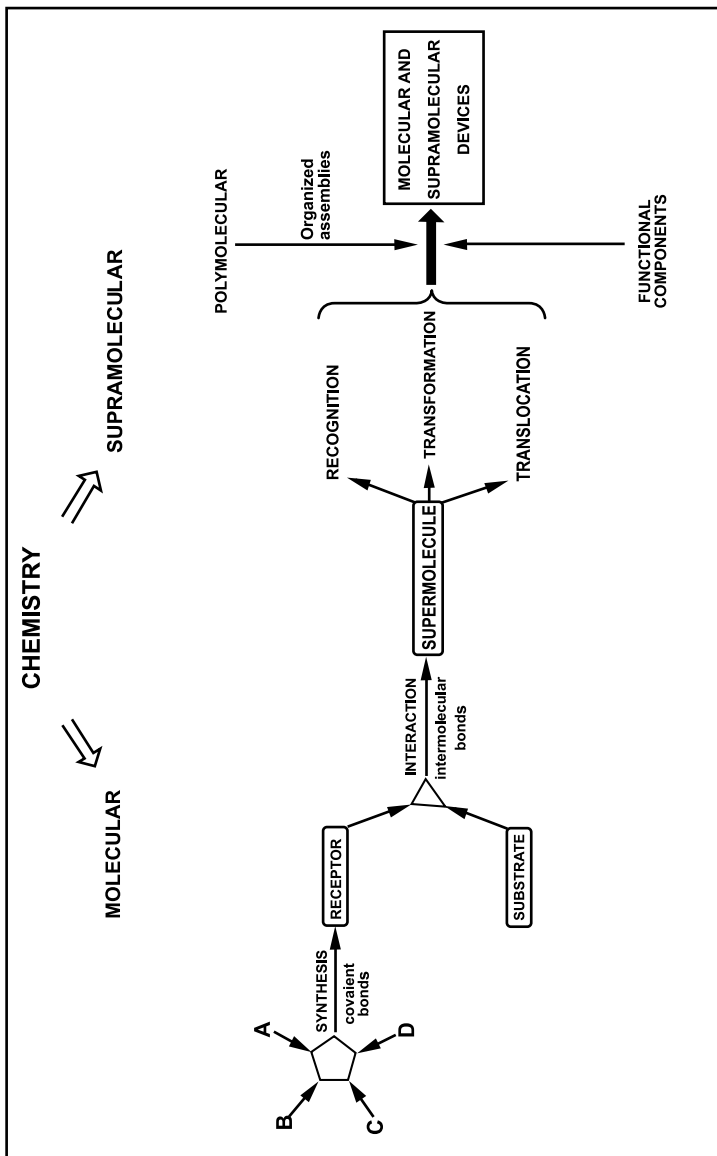
Figure 2: From Molecular to Supramolecular Chemistry: molecules, supermolecules, molecular and supramolecular devices.
